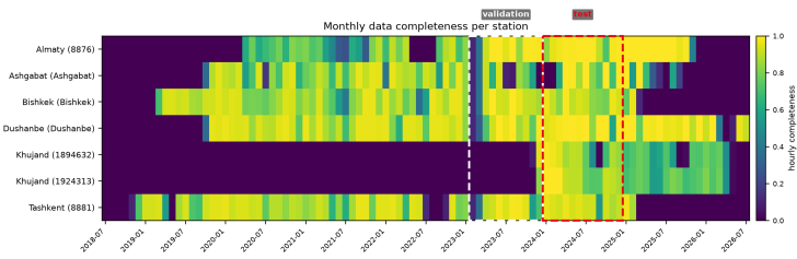
Figure 2. Monthly hourly-completeness for each of the 7 benchmark stations. Dashed boxes mark the validation (2023-01-11 to 2023-12-21) and test (2024-01-01 to 2024-12-31) blocks. Both Khujand sensors begin on 2023-11-28 and 2023-12-06, after the training block closes, and the record ends unevenly, with 2 of 7 stations, Bishkek and Tashkent (8881), stopping at the StateAir closure on 2025-03-04 while the remainder continue through a longer-lived feed. All of that lies beyond the test block and none of it is used.
